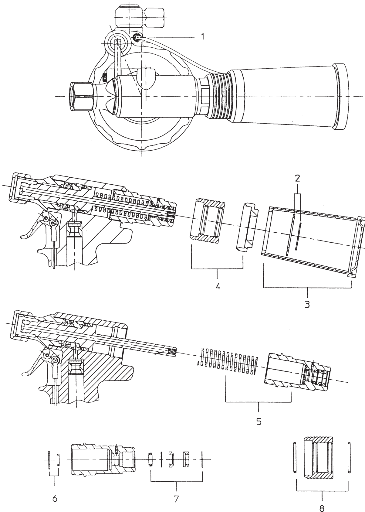
Exploded View of Vacuum Attachment
